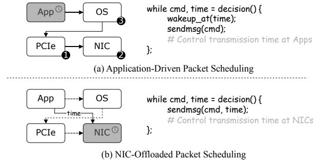
Figure 21: Comparison of packet transmission timing control methods on end devices.
