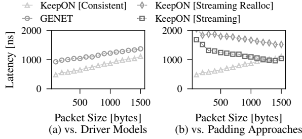
Figure 10: Comparison of total driver transmit path latency. (a) Median delay of KeepON and GENET. (b) Median delay of different padding approaches, comparing streaming DMA (w/o sufficient tailroom) versus consistent DMA.
